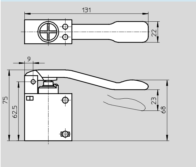
Finger lever valve TH-3-1/4-B, TH0-3-1/4-B
