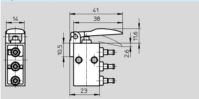
Finger lever valve TH/0-3-PK-3
