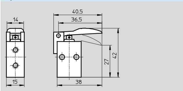
Finger lever valve TH-3-M5
