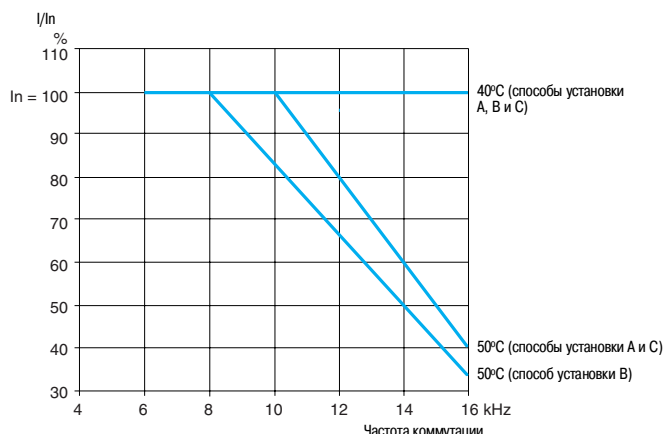
ATV 21HU22N4
