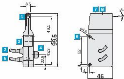
Dimensional drawing WLR2-P610SC1
