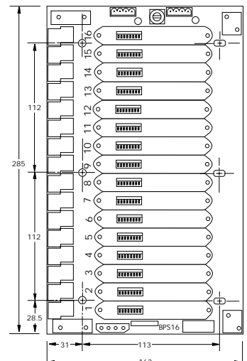
BPS16 16-way backplane (screw-clamp connectors)
